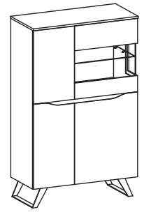
MA-KB barek L,P W:1455 S:900 G:420
