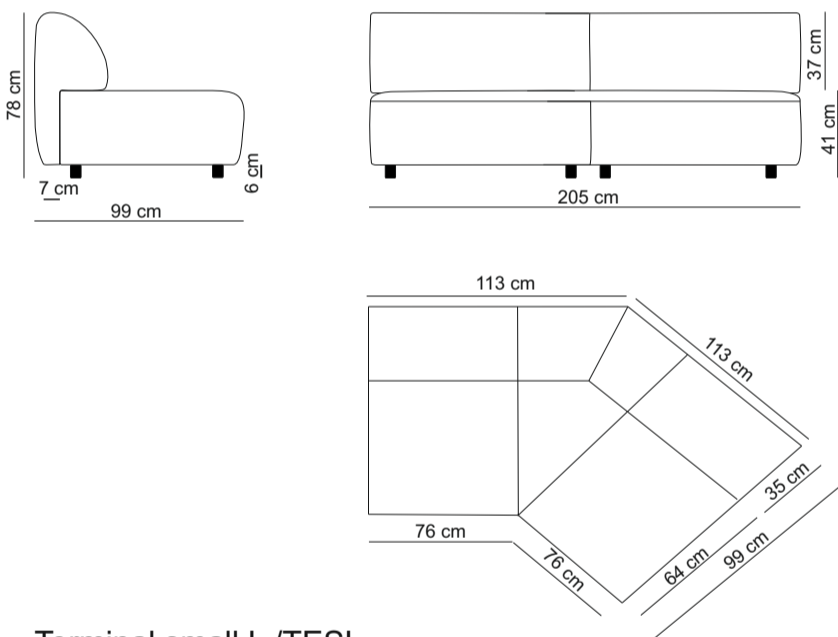
Terminal small L /TESL
